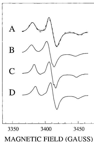
FIGURE 4 ( A ) Effective powder ESR spectra of DPPTC in ISDU-aligned DPPC membranes in the presence of excess water. —, Experimental; - - -, simulated. The best fit parameters of the g and A tensor components obtained from this simulation were used for fitting the ESR spectra in Fig. 5. ( B ) Experimental rigid limit ESR spectrum of 16PC in DPPC dispersions. ( C and D ) Effective powder ESR spectra of 16PC in pressure-annealed and ISDU-aligned DPPC bilayers, respectively.
