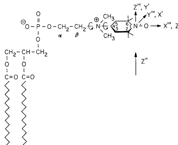
FIGURE 3 The structure of phosphoryl-tempo-choline in DPPTC and the various axis systems defined for the spectral simulations (see text).
